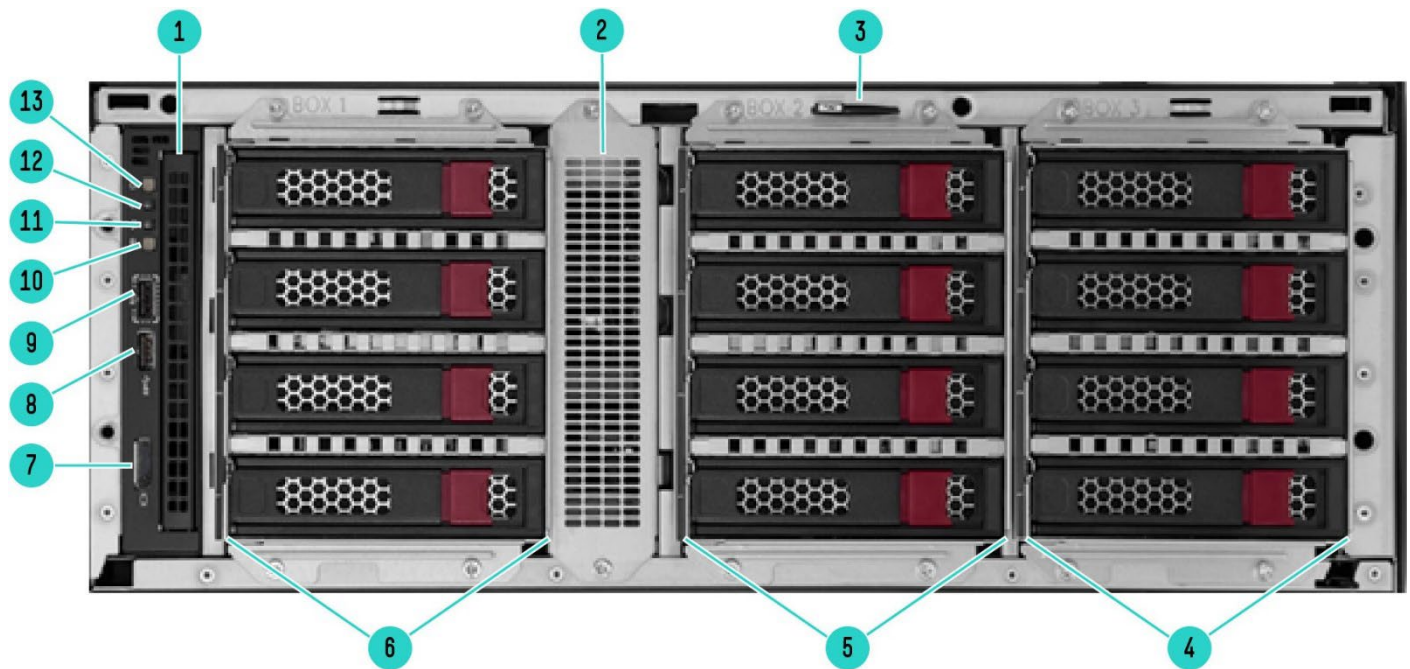
Front View – LFF chassis with optional Gen11 4LFF HDD Cage Kits shown (Rack mode)
